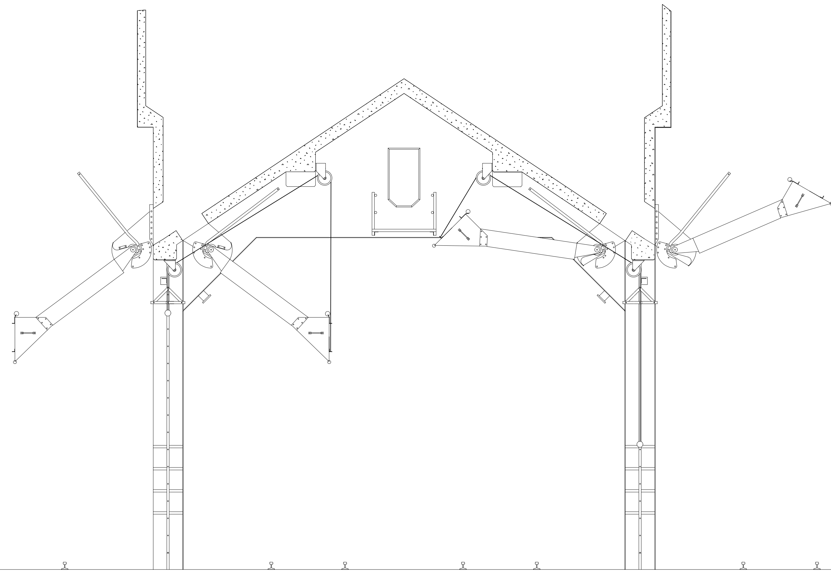
SECTION THROUGH EAST BAY OF COAL DOCK
