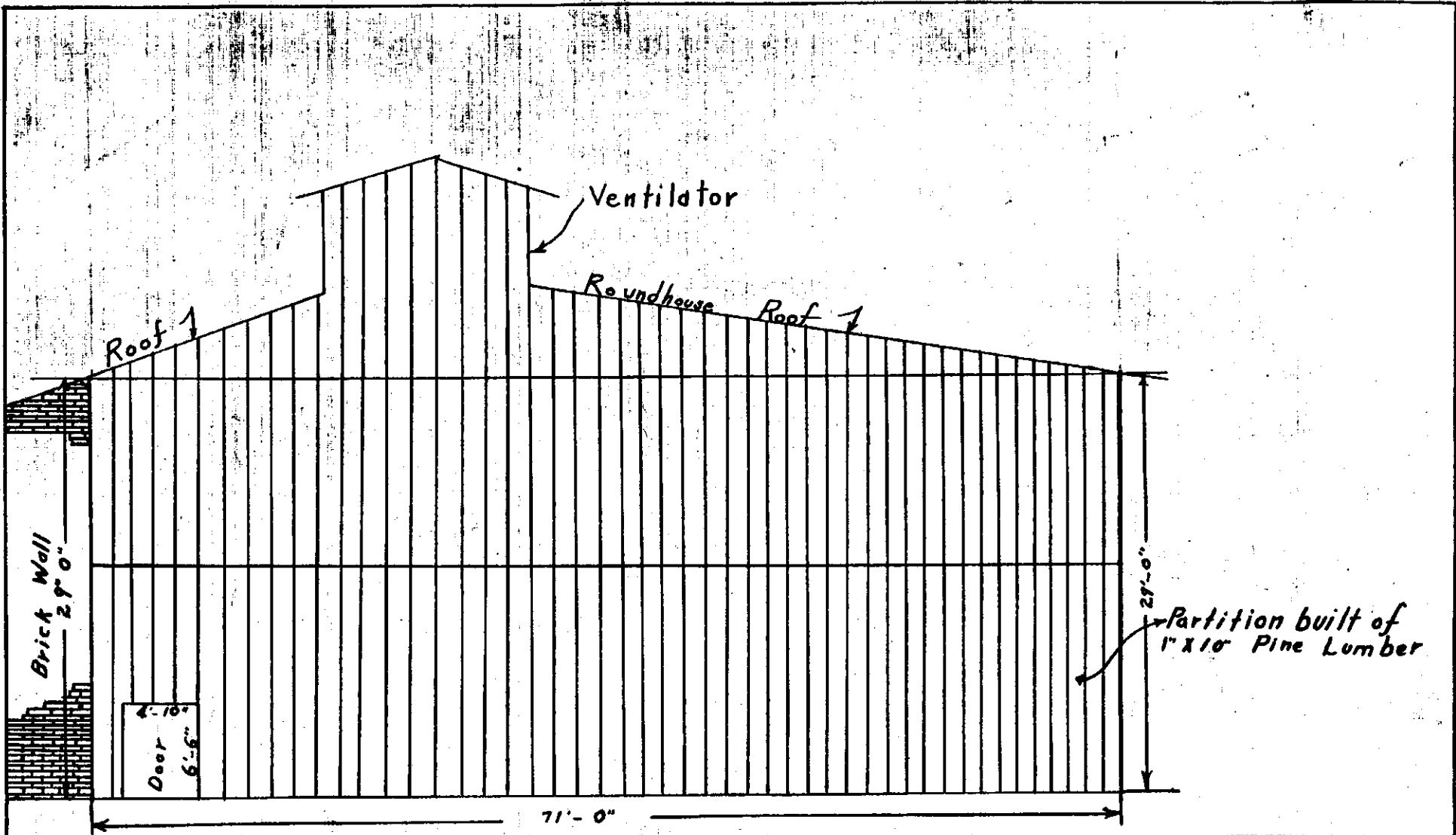
CROSS SECTION
