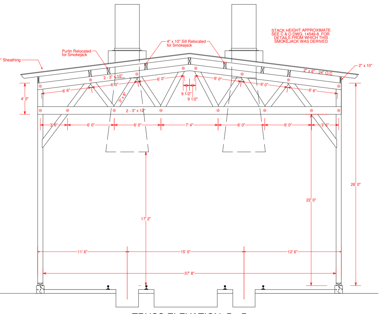
TRUSS ELEVATION B - B
