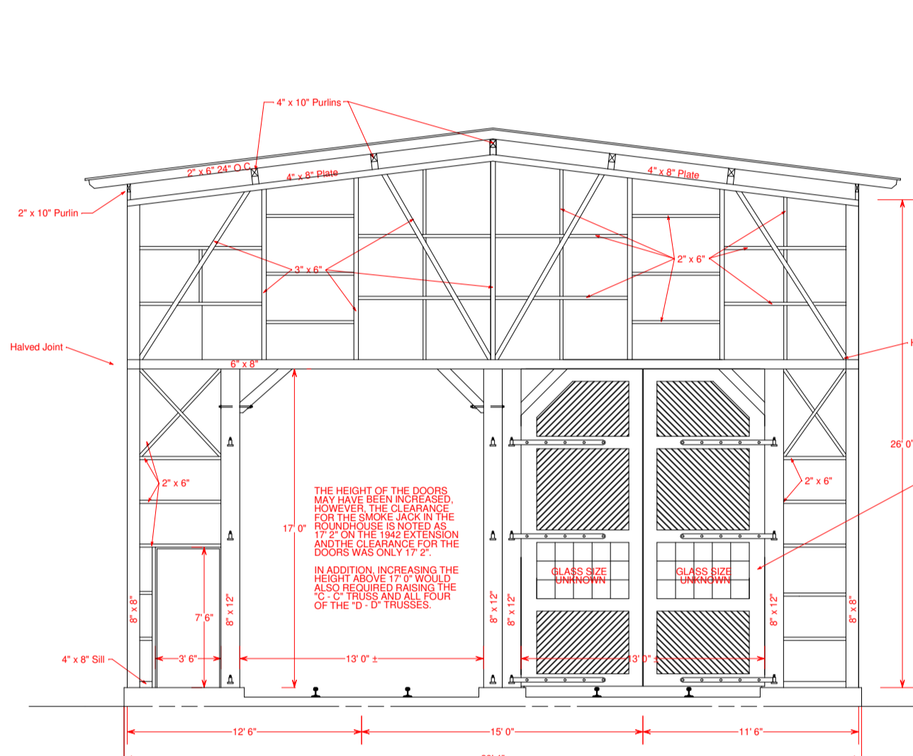
EAST ELEVATION A - A (FRAMING)
