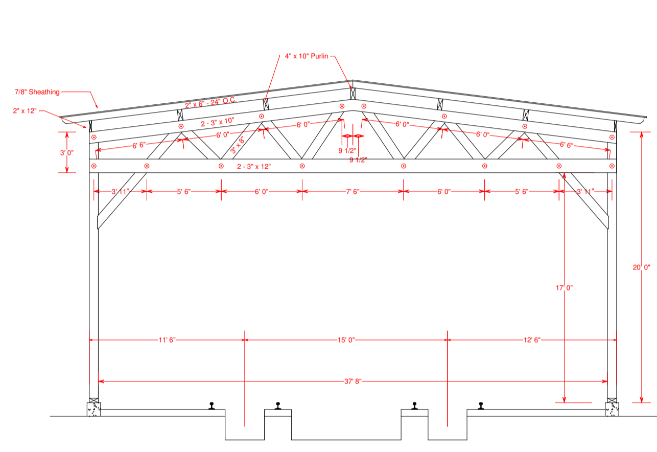
TRUSS ELEVATION D - D
