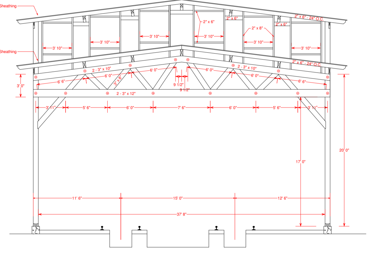
TRUSS ELEVATION C - C
