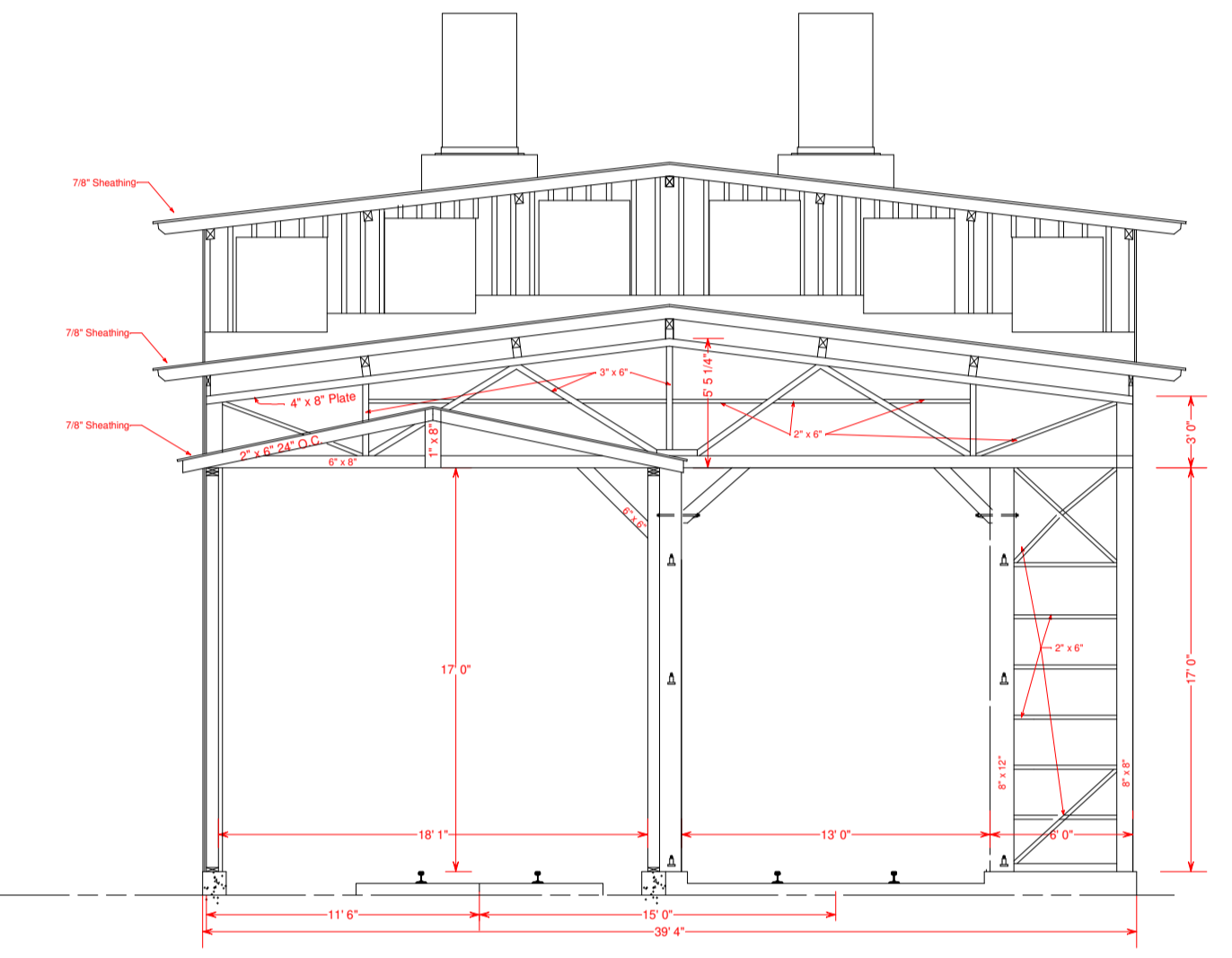
WEST ELEVATION E - E (FRAMING)
