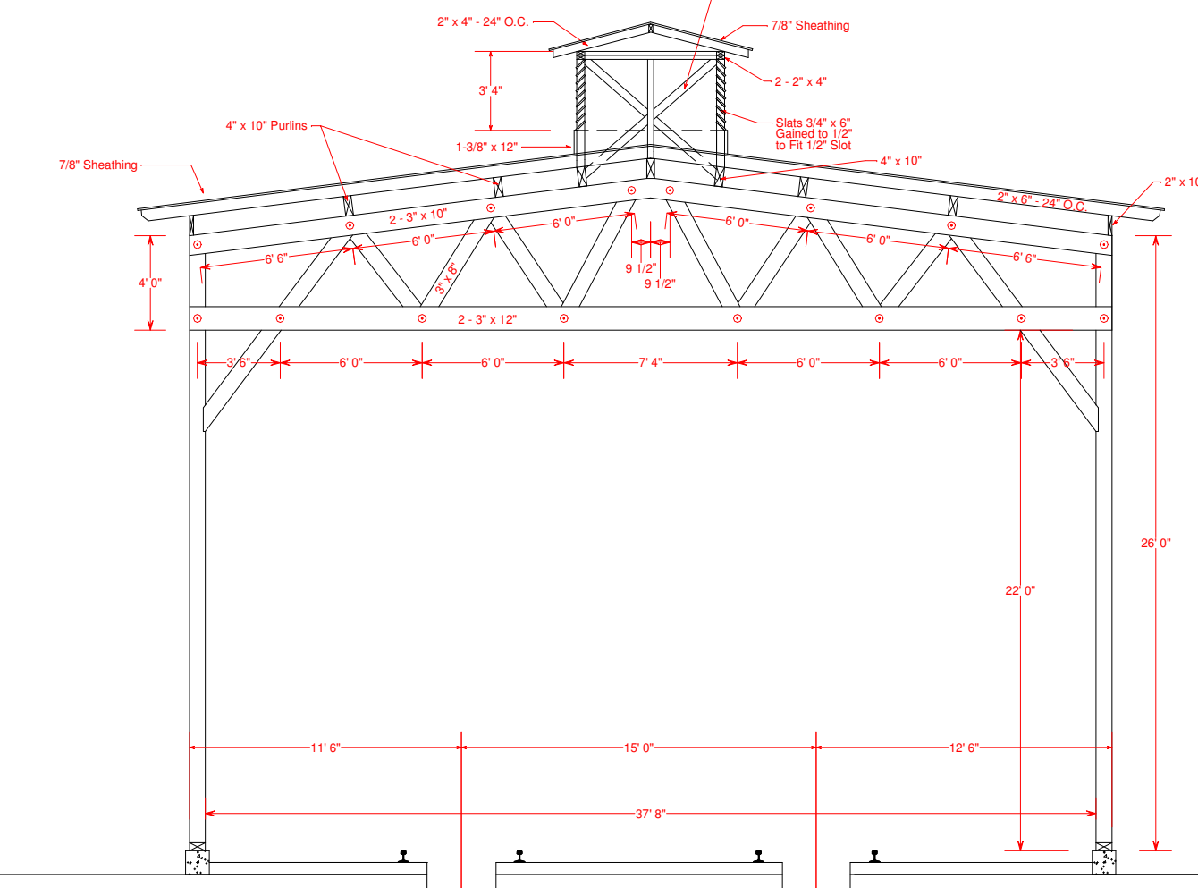
TRUSS ELEVATION B - B
