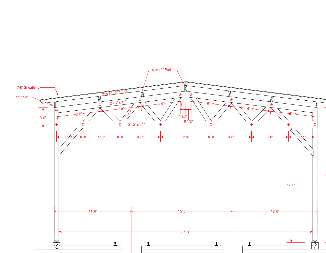
TRUSS ELEVATION D - D
