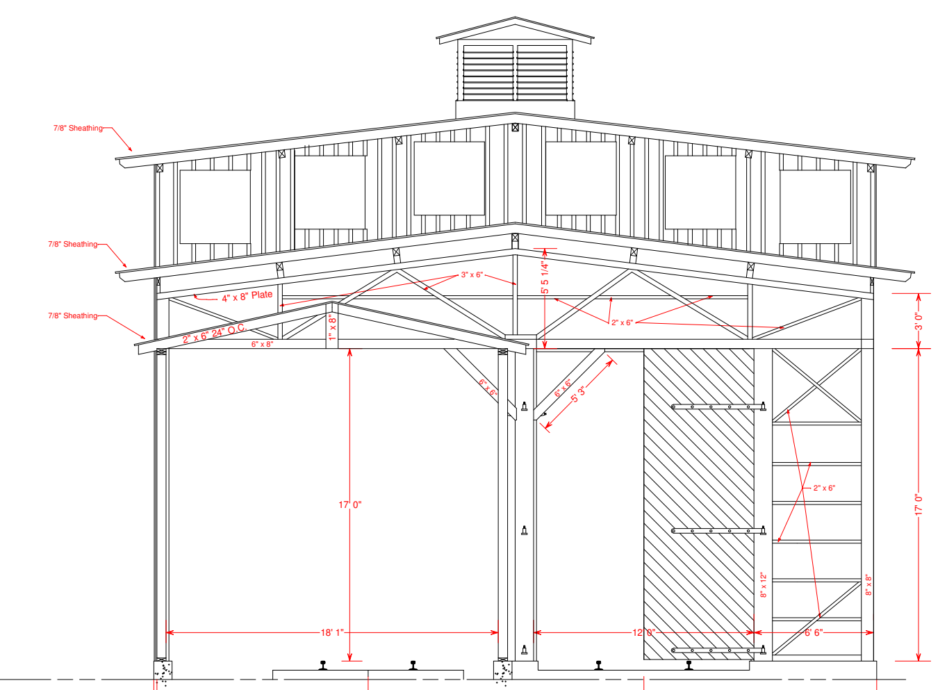
WEST ELEVATION E - E (FRAMING)
