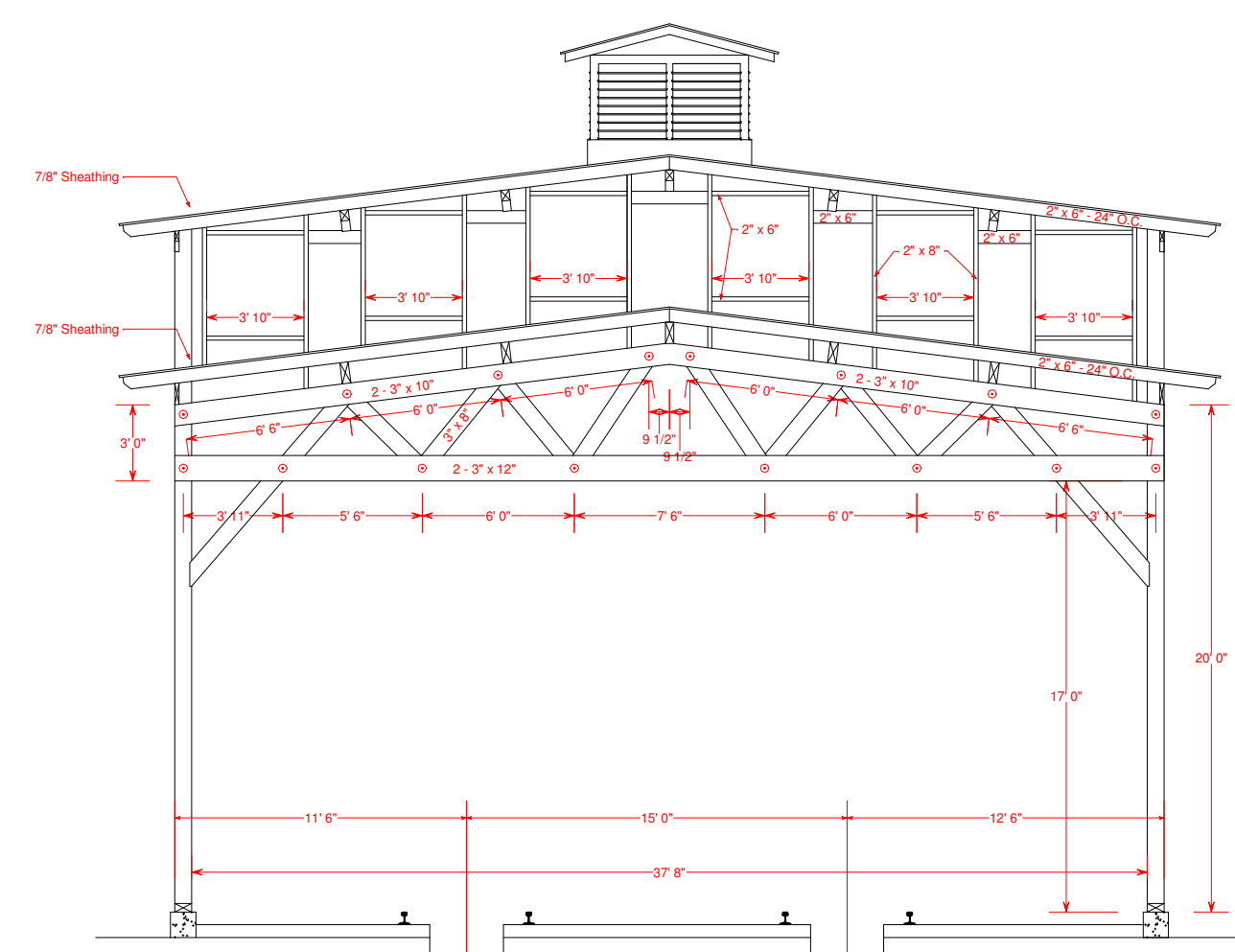
TRUSS ELEVATION C - C
