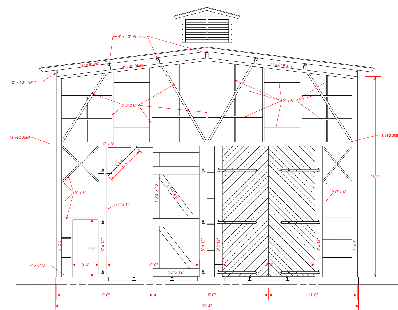
EAST ELEVATION A - A (FRAMING)
