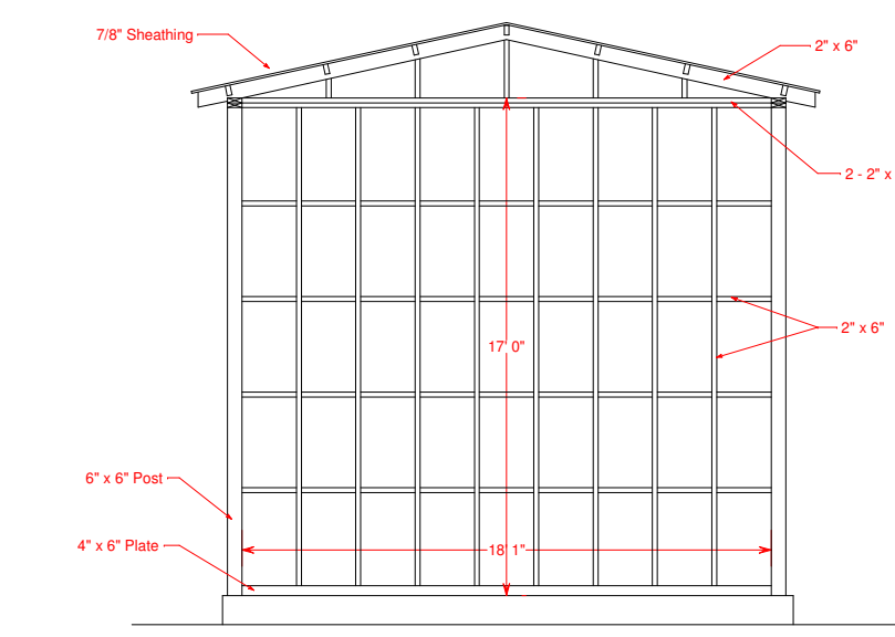
WEST END CARPENTER SHOP Extrapolated from C & O Drawings and Standard Practices
